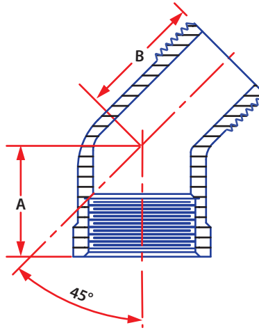
45° Elbow - Street
