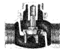
Lift Check Cutaway
