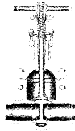
Buttweld Cutaway
